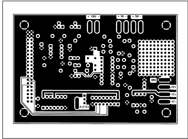
Figure 6. MAX110 EV Kit PC Board Layout—Solder Side
